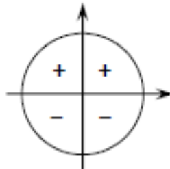
\sin t
